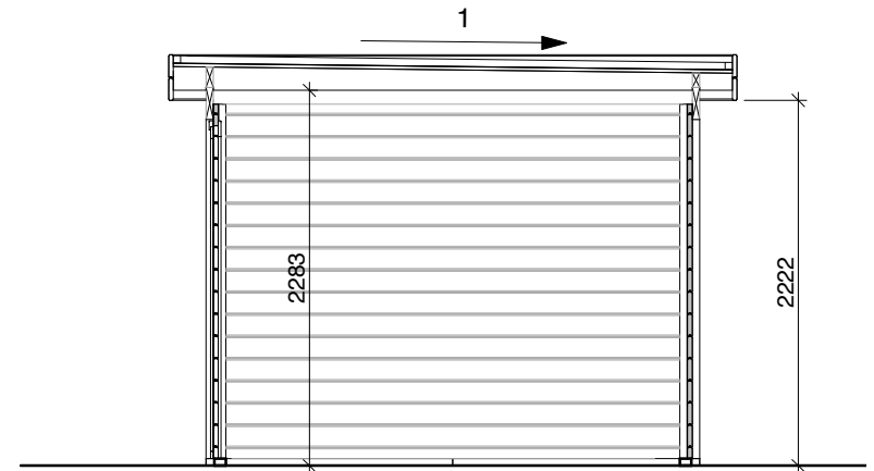
SECTION 1-1
