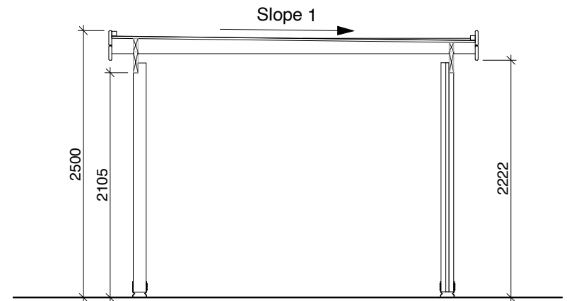
SECTION 1-1
