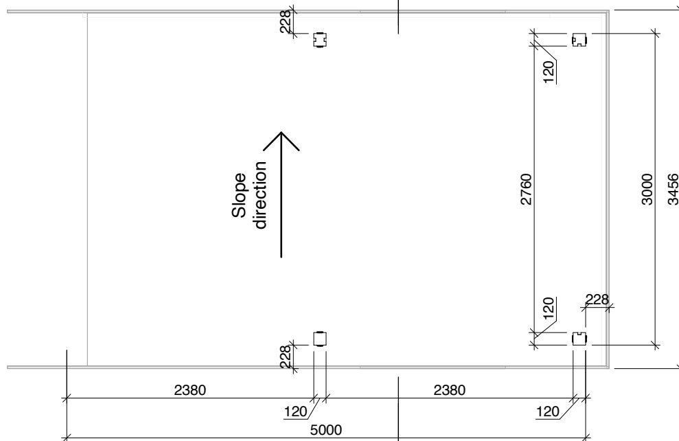
FLOOR PLAN
